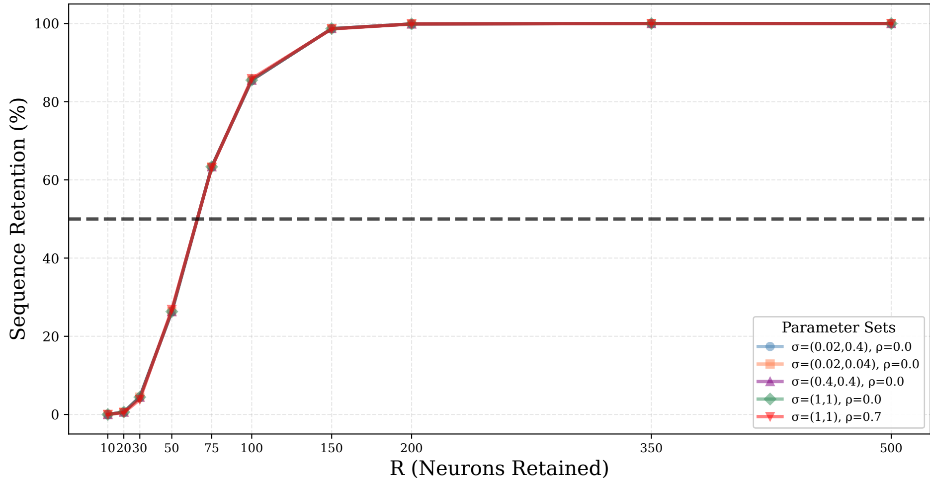
Sequence Retention vs Subsampled Neuron Count (R) with 50% Sequence Retention Reference | v=(0.07, 0.9)
