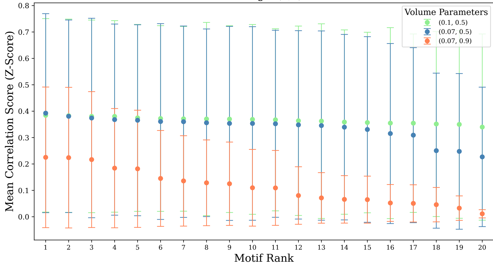
Mean Correlation Scores per Motif of One Subsample (Independently Ranked) \sigma Range: (1,1)
