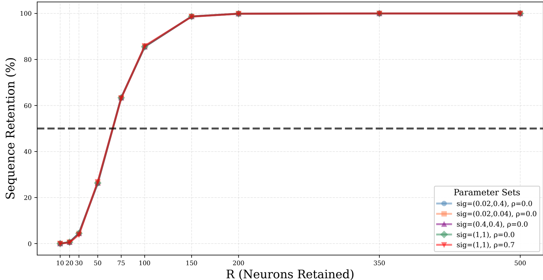
Sequence Retention vs Neuron Threshold (R) with 50% Retention Reference
