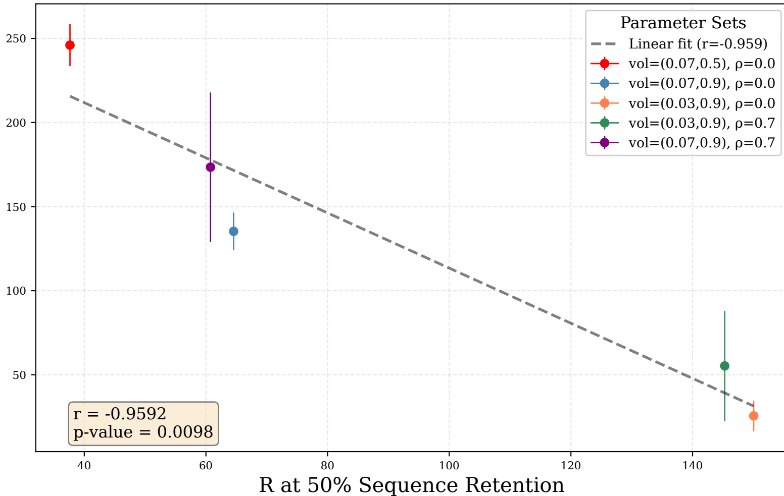
Average Neuron Participations vs R where Sequence Retention Crosses 50% sigma=(0.02, 0.4) | Pearson correlation applied
