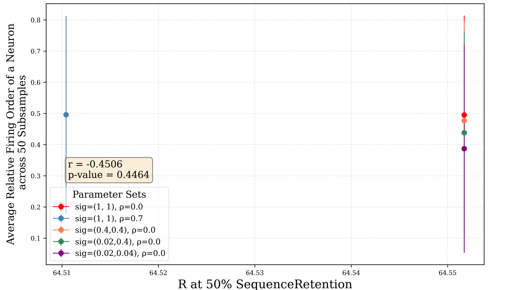
Average Relative Firing Order of a Neuron at R where Sequence Retention Crosses 50% vol=(0.07, 0.9) | Pearson correlation applied
