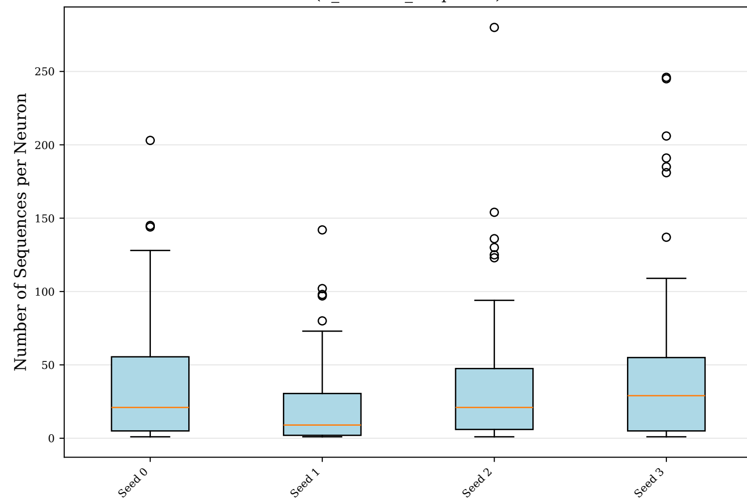
Sequence Participation Distribution by Seed (n_neurons_keep=100)
