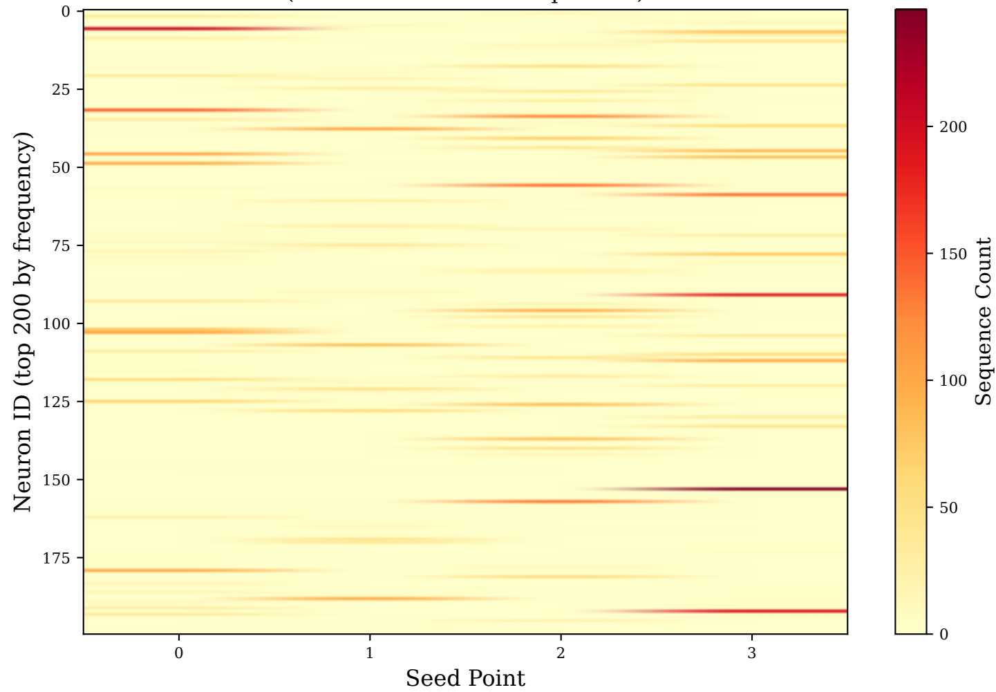
Neuron Participation by Seed (Color = Number of Sequences)
