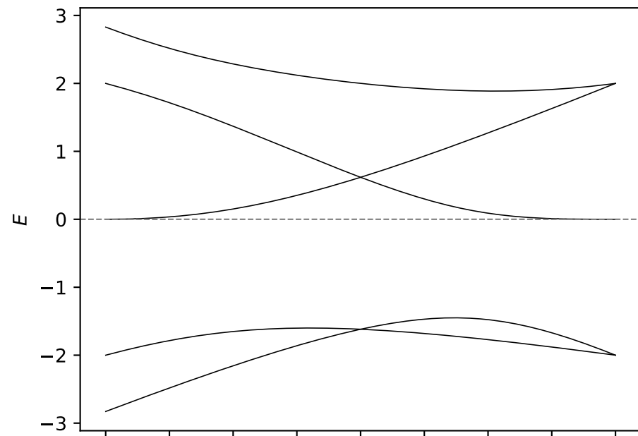
N = 25 (PBC)
