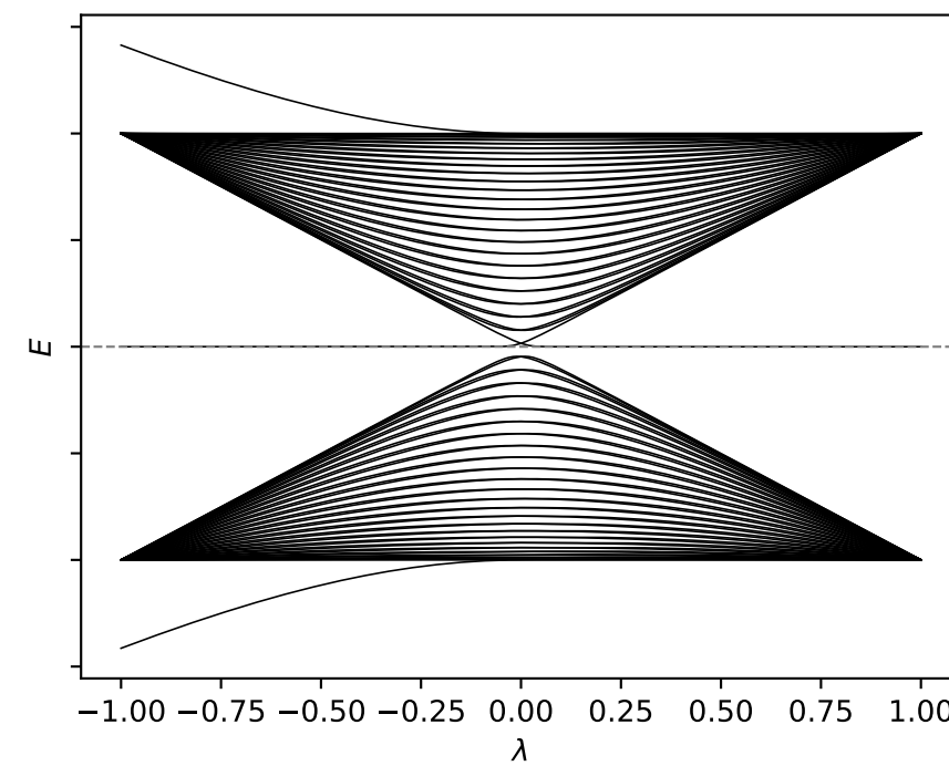
N = 101 (PBC)
