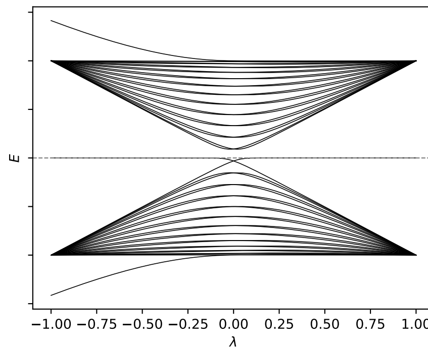
N = 51 (PBC)
