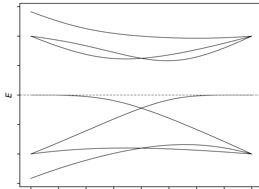
N = 51 (PBC)
