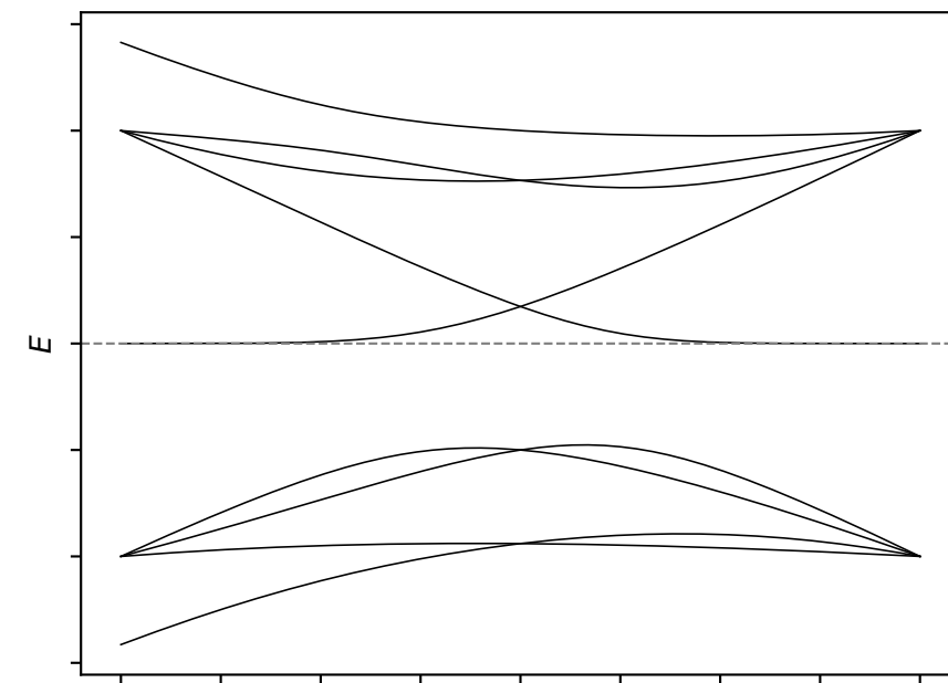
N = 101 (PBC)
