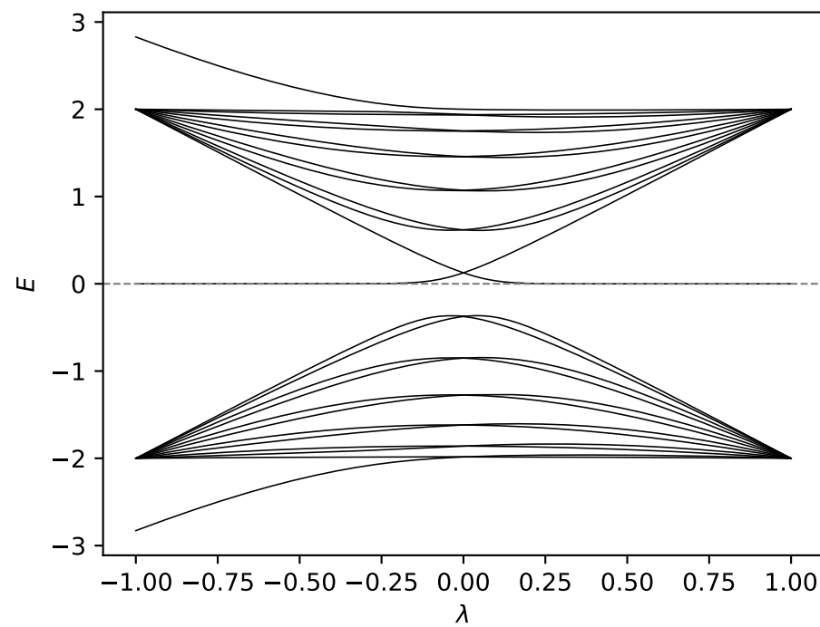
N = 25 (PBC)
