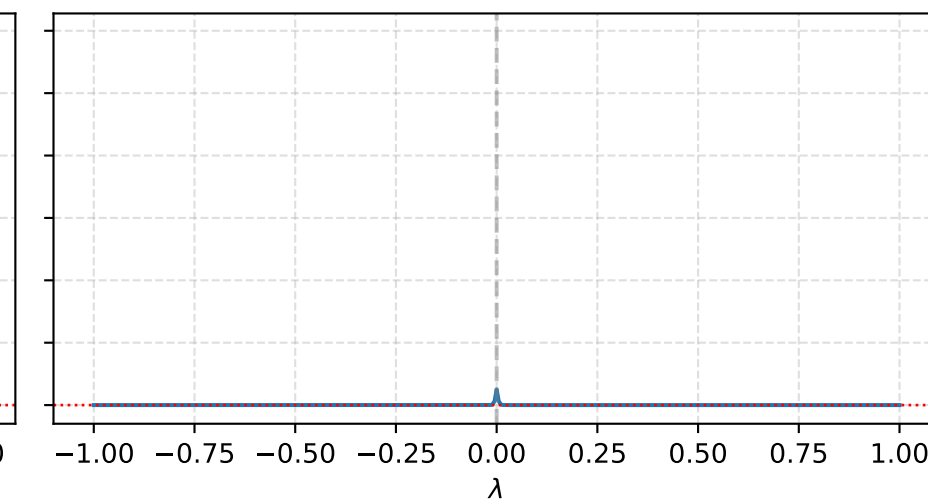
N = 501 (PBC)
