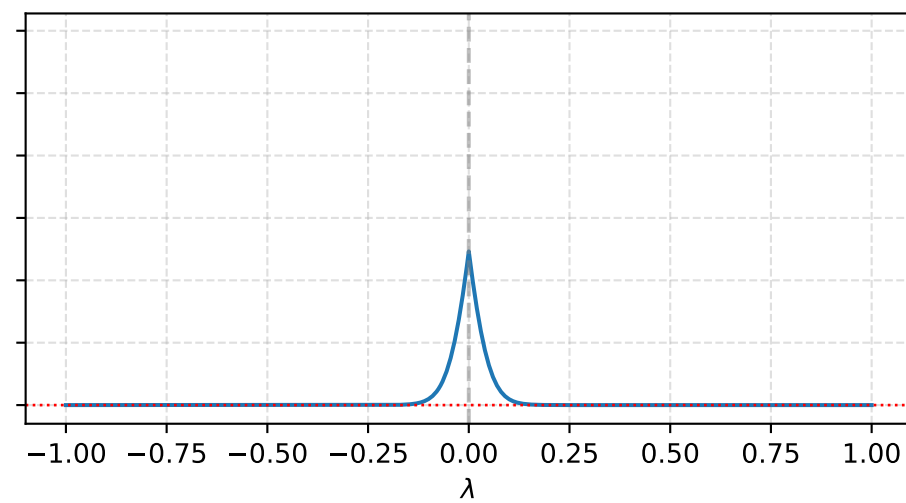
N = 51 (PBC)
