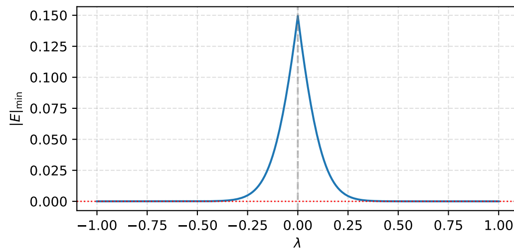
N = 21 (PBC)
