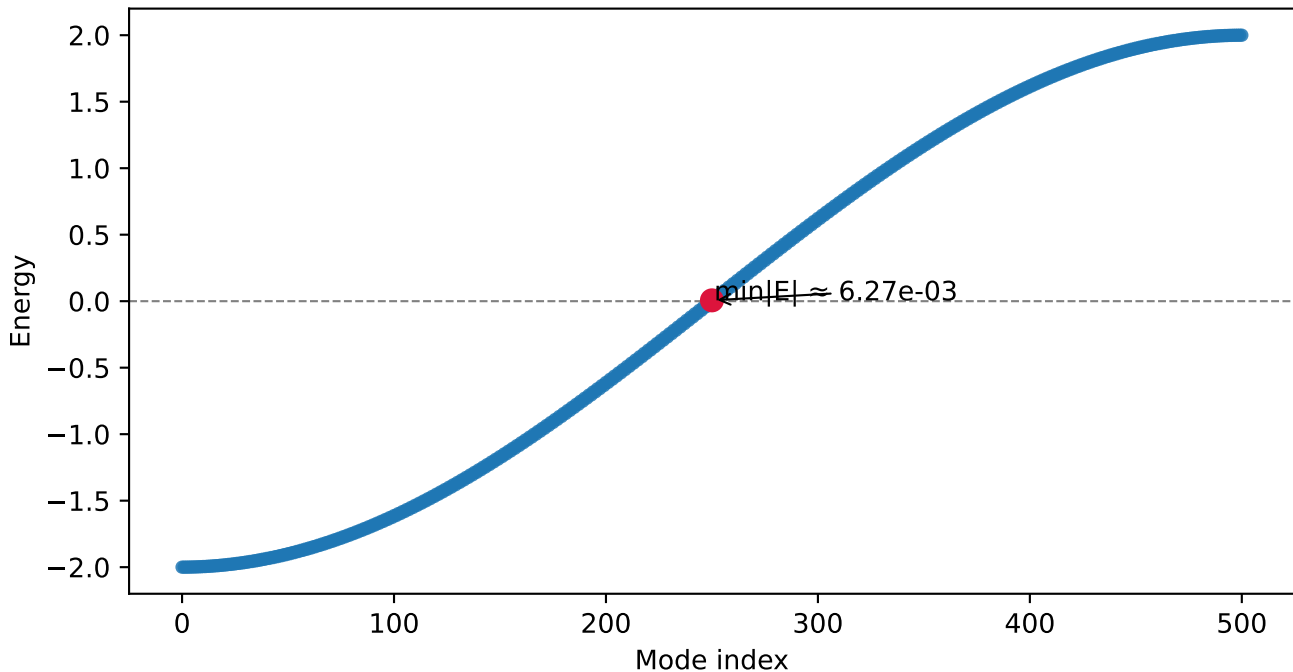
SSH Spectrum (N=501, \lambda=0.0 , PBC)
