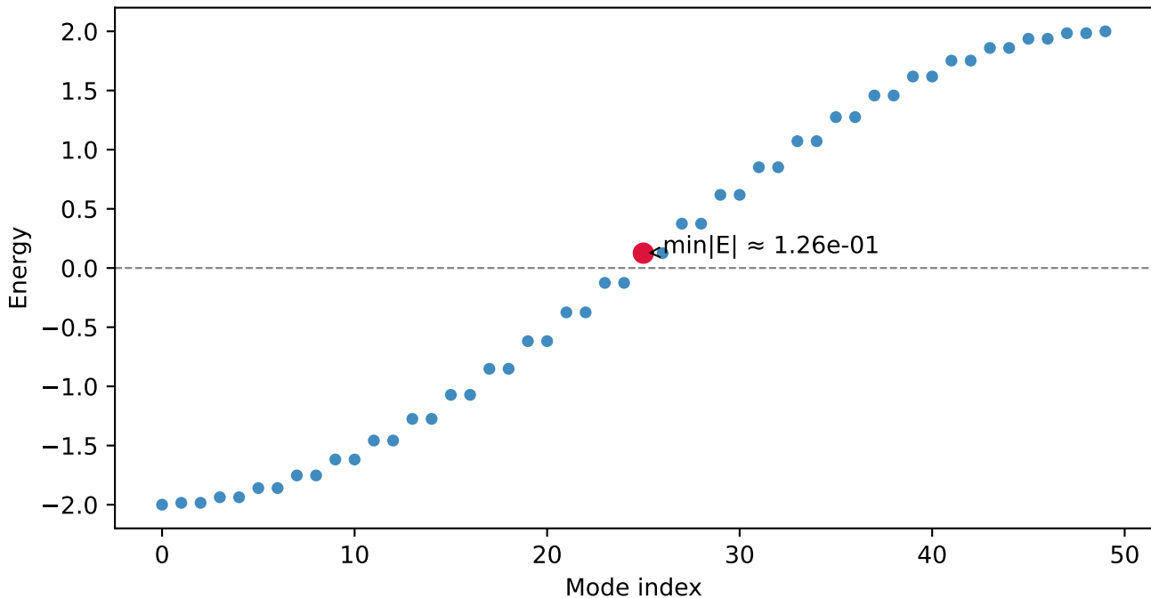
SSH Spectrum (N=50, \lambda=0.0 , PBC)
