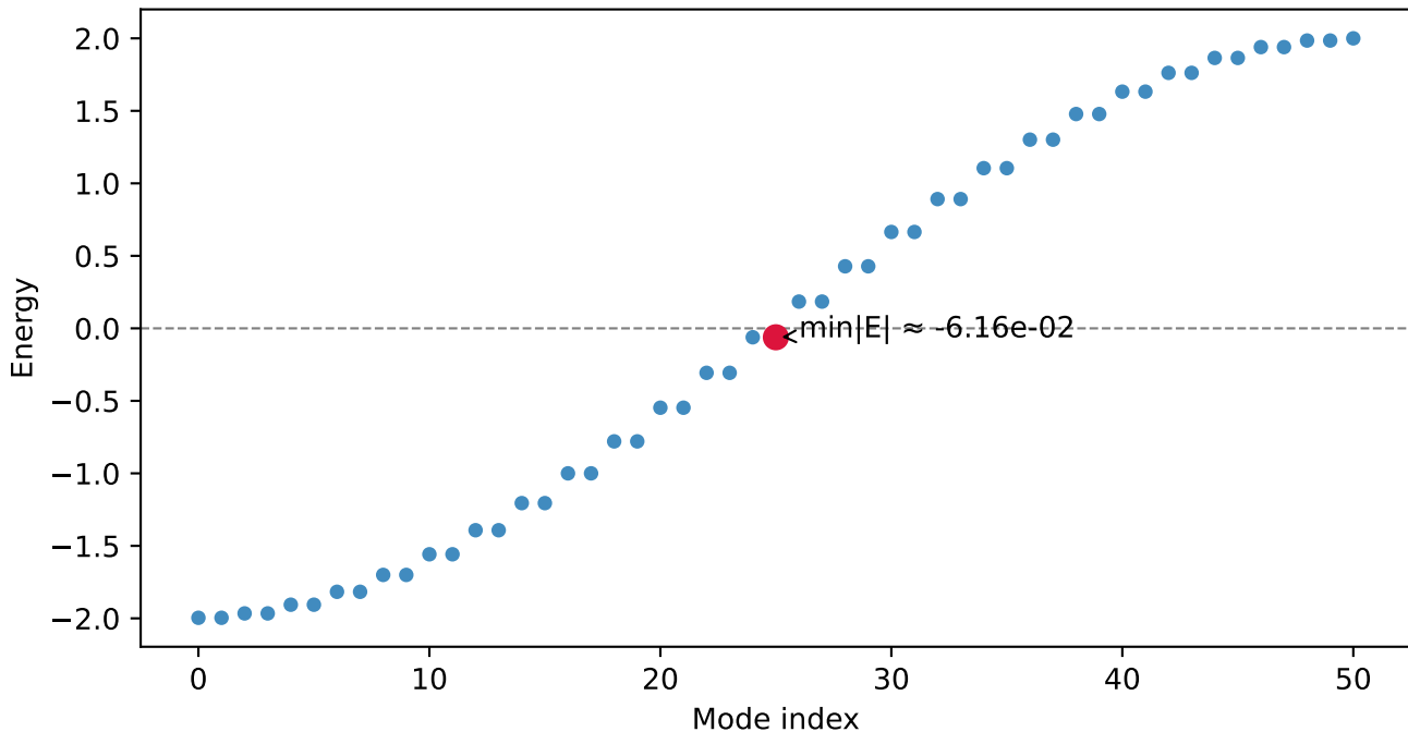
SSH Spectrum (N=51, \lambda=0.0 , PBC)
