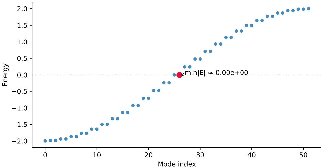
SSH Spectrum (N=52, \lambda=0.0 , PBC)
