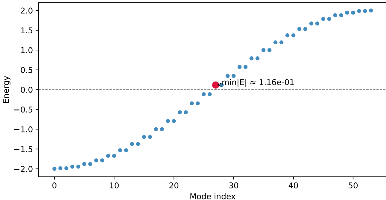
SSH Spectrum (N=54, \lambda=0.0 , PBC)
