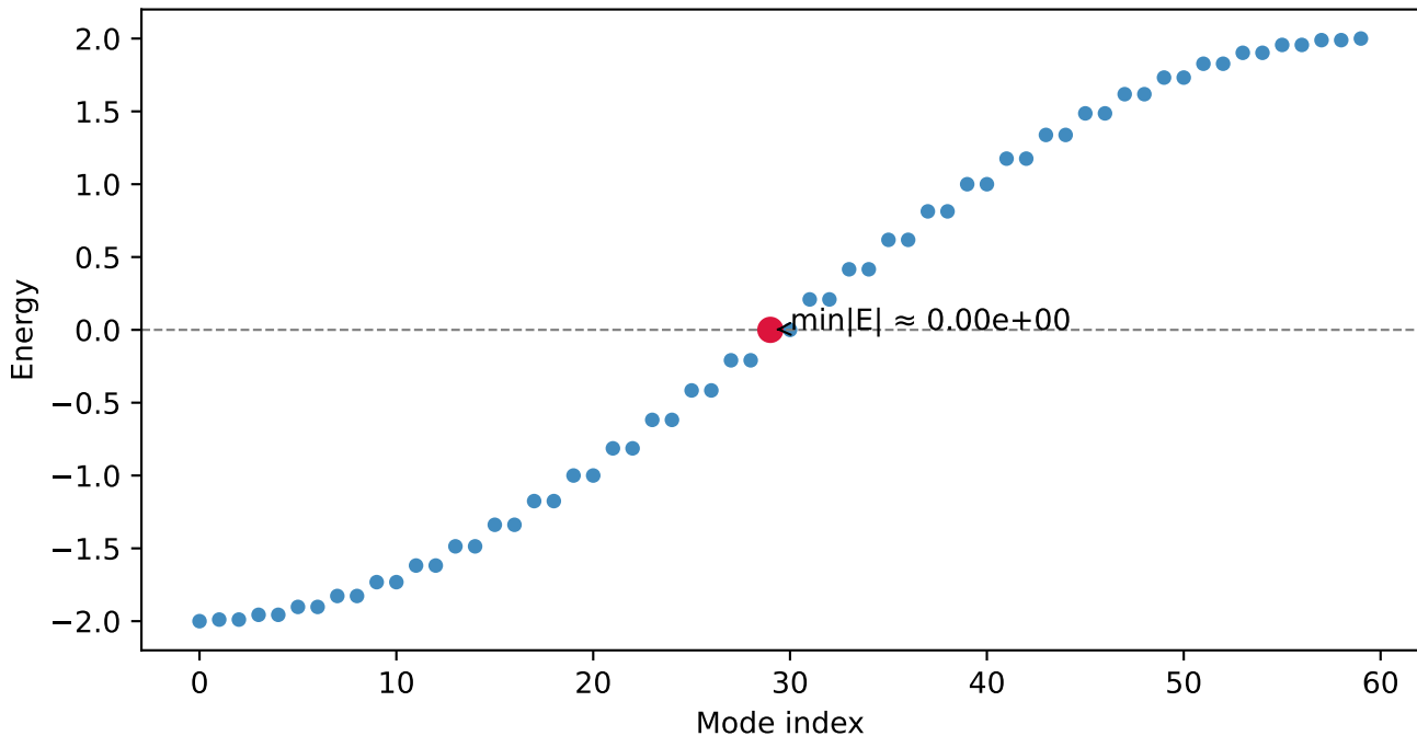
SSH Spectrum ( N=60 , \lambda=0.0 , PBC)
