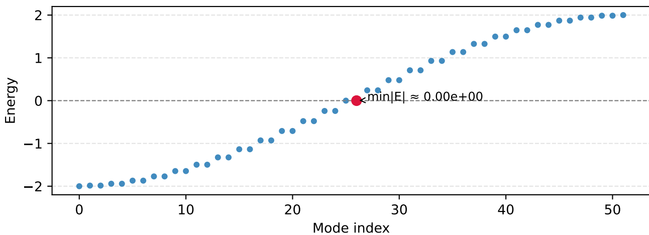
N = 52, \lambda = 0.0 (PBC)
