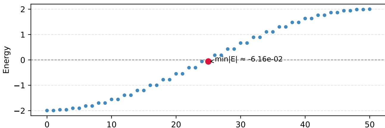
N = 52, \lambda = 0.0 (PBC)
