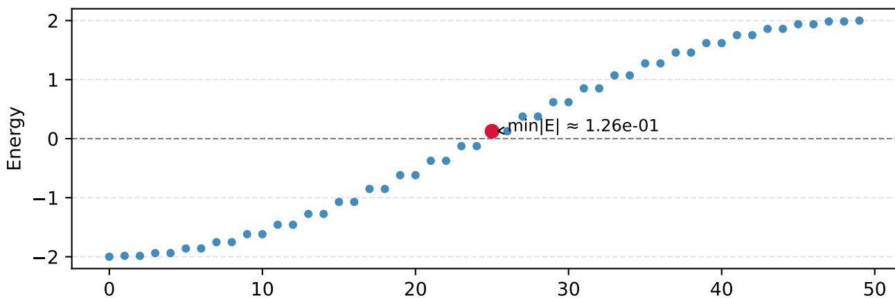
N = 51, \lambda = 0.0 (PBC)
