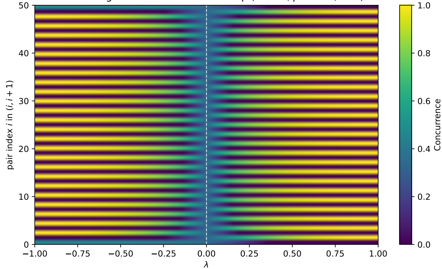
Nearest-neighbor concurrence heatmap ( N = 51 , \beta = 30.0 , PBC)
