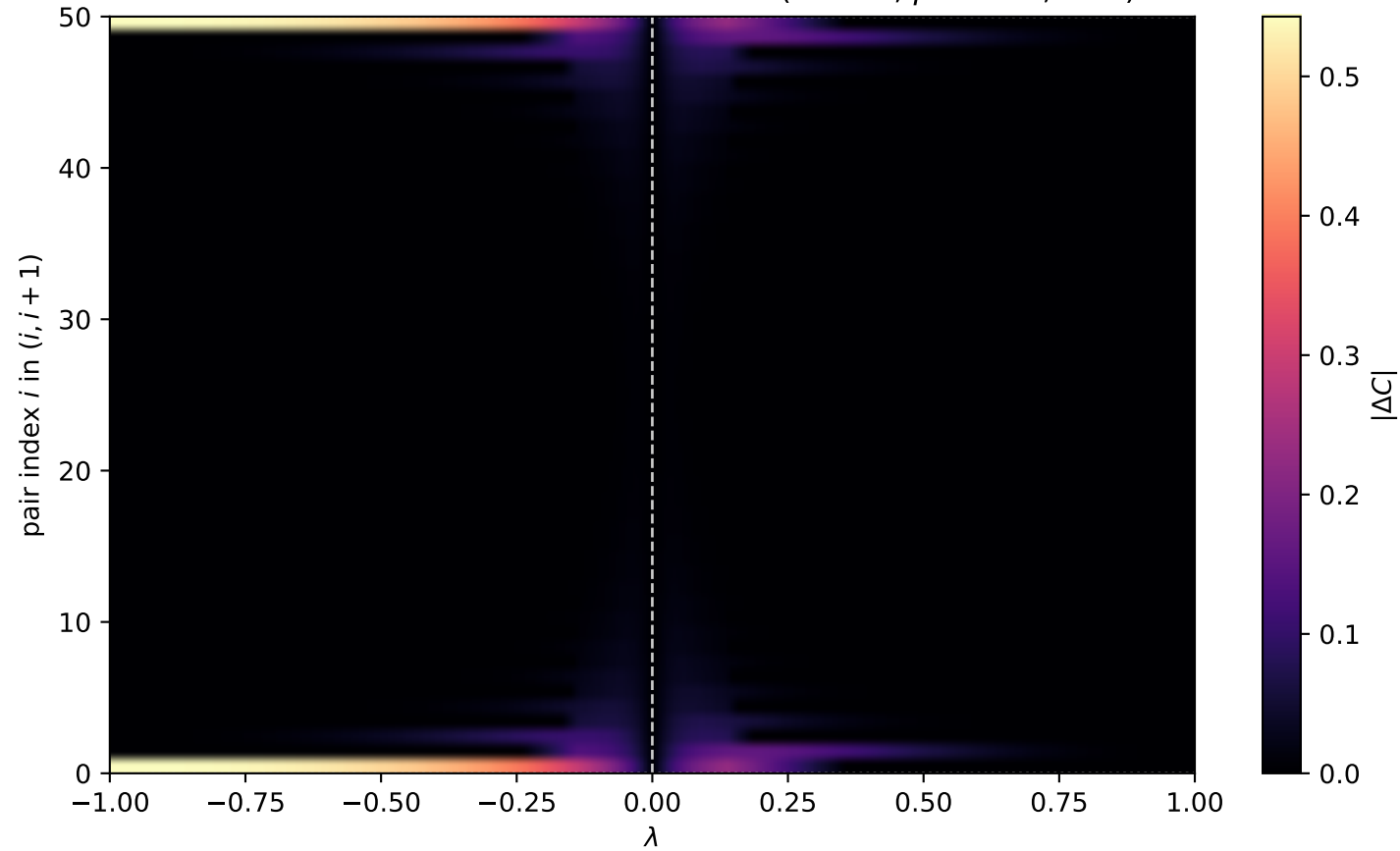
Defect-induced concurrence deviation ( N = 51 , \beta = 30.0 , PBC)
