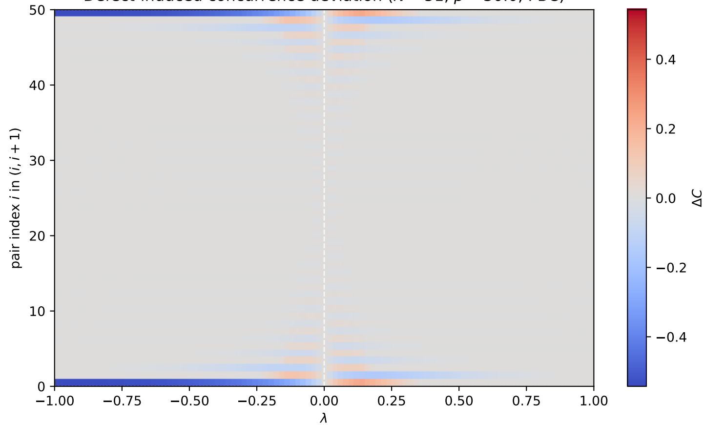
Defect-induced concurrence deviation ( N = 51 , \beta = 30.0 , PBC)
