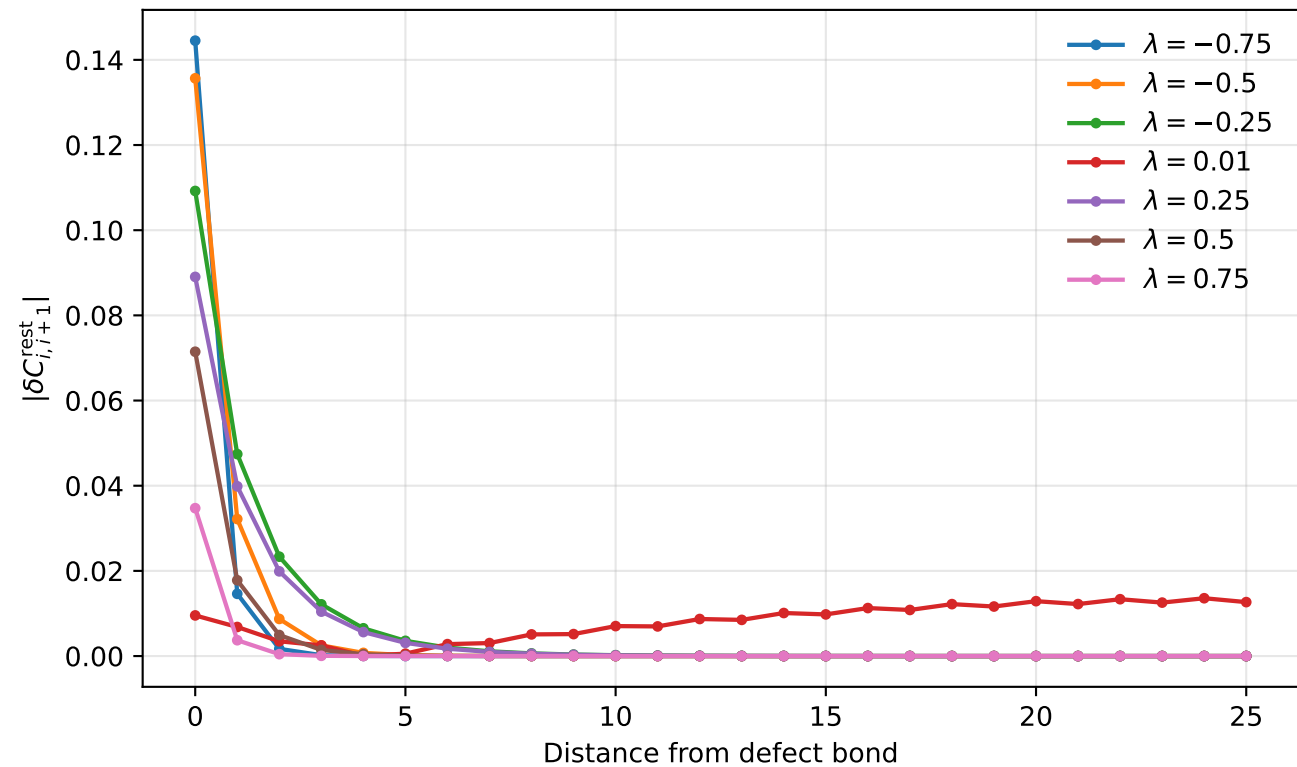
Background deformation vs distance ( N = 51 , \beta = 30.0 )
