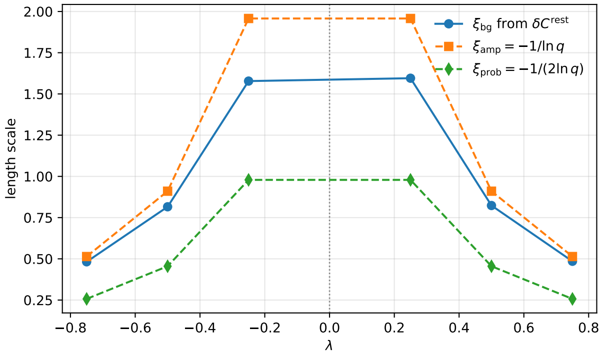
Background deformation length vs zero-mode length ( N = 51 , \beta = 30.0 )
