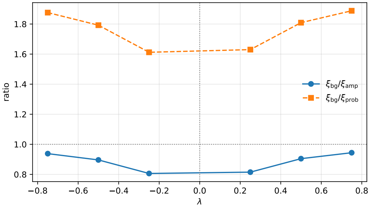
Background length relative to zero-mode length
