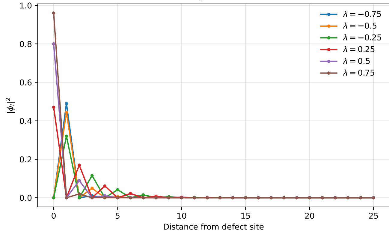
Trial near-zero mode profile vs distance ( N = 51 )
