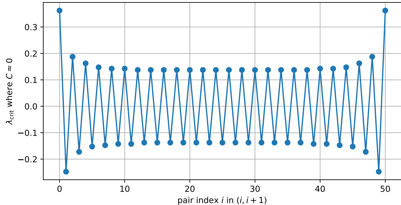
Critical \lambda vs pair index ( N=51 , \beta = 30.0 , Periodic)
