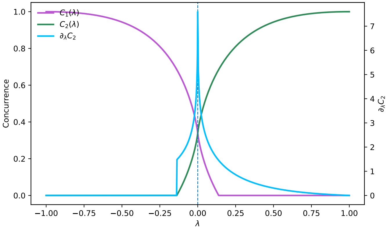
Wootters concurrence (T=0)
