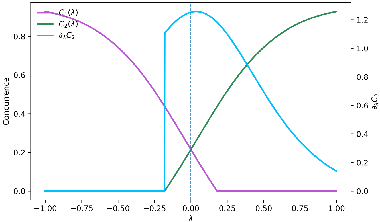
Wootters concurrence ( \beta = 2 )
