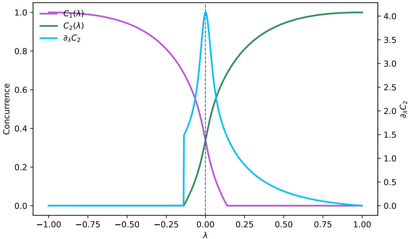
Wootters concurrence ( \beta = 30 )
