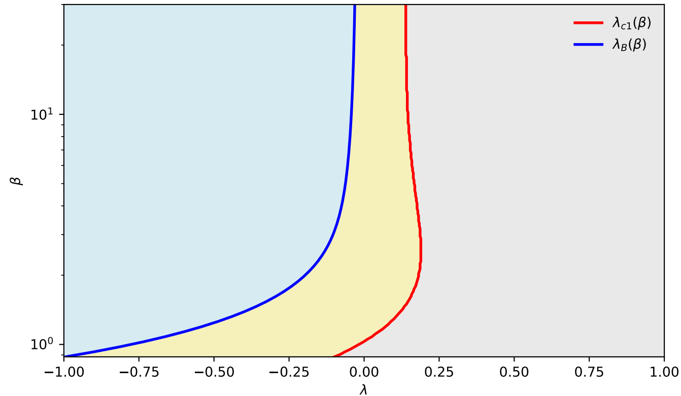
Phase diagram from concurrence and Bell violation ( r = 0 )
