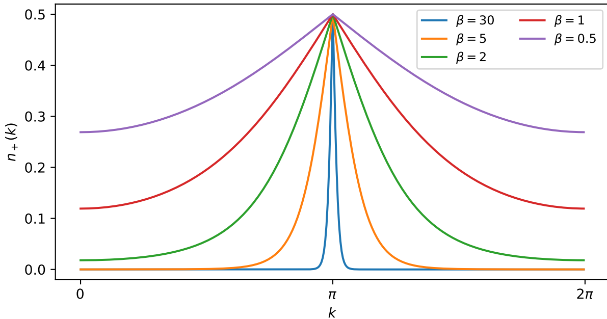
Upper band occupation n_+(k) (fixed \lambda = 0.0 )
