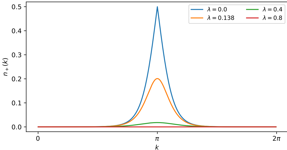
Upper band occupation n_+(k) (fixed \beta = 5.0 )
