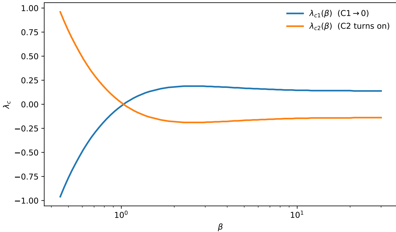
Critical \lambda_c(\beta) from concurrence
