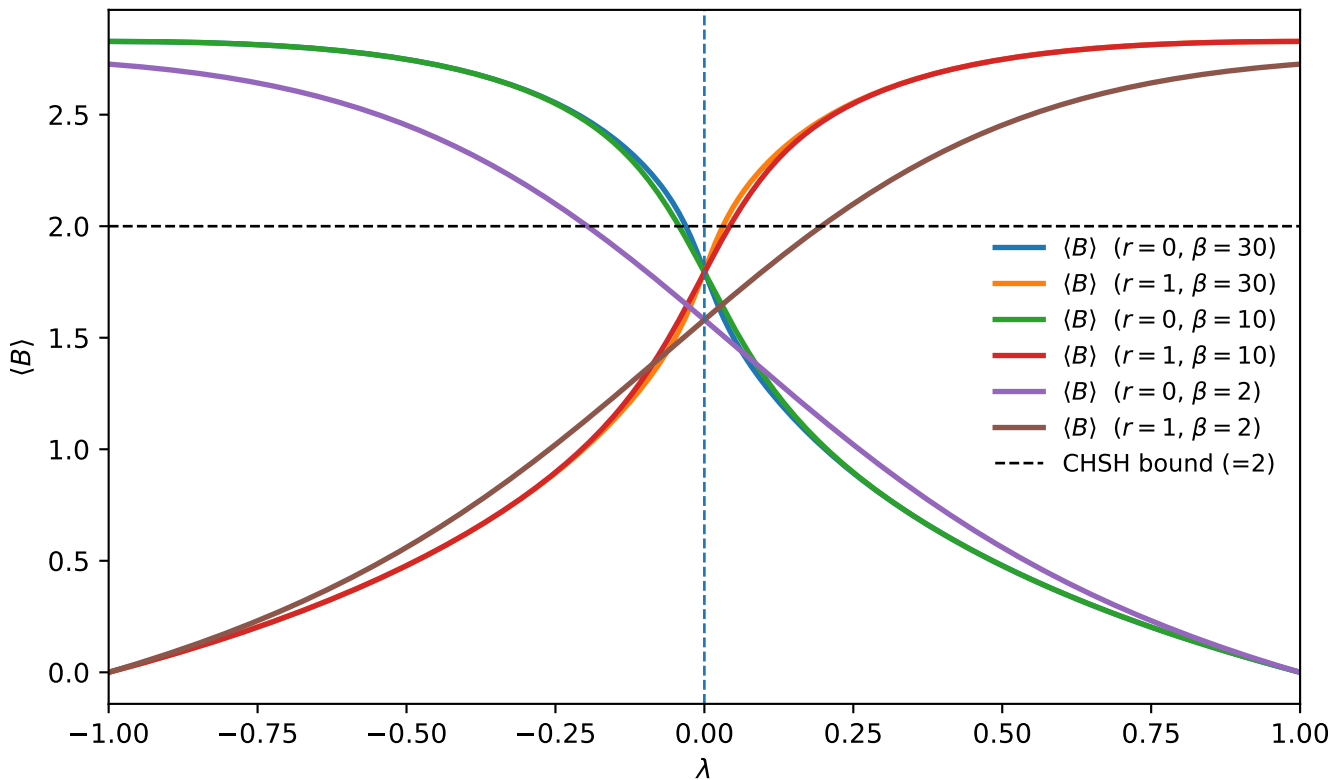
Bell expectation \langle B \rangle vs \lambda
