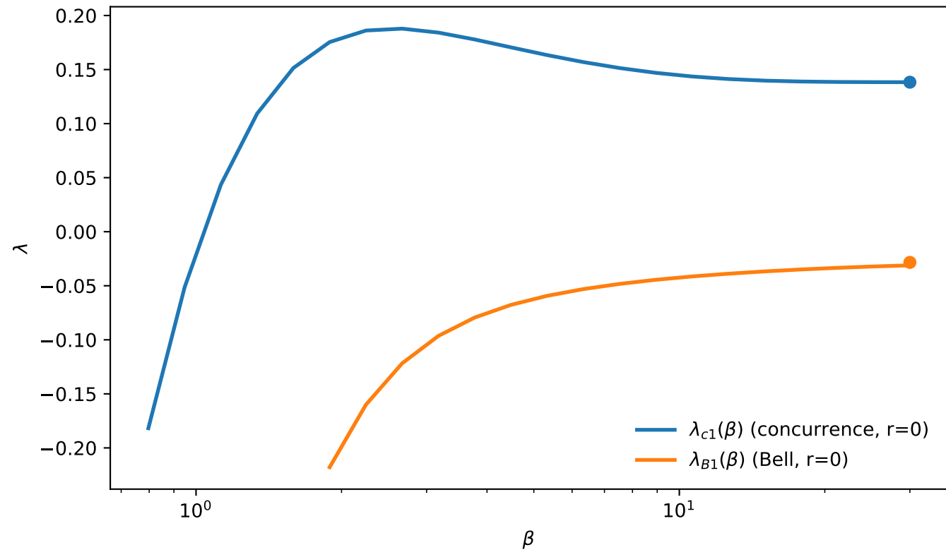
Phase boundaries (r=0): concurrence vs Bell violation
