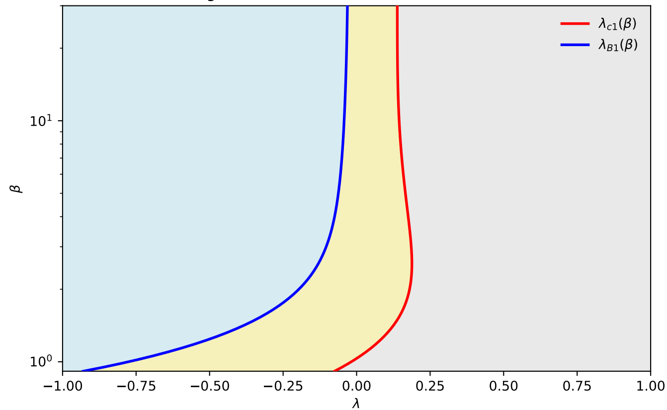
Phase diagram from concurrence and Bell violation ( r=0 )
