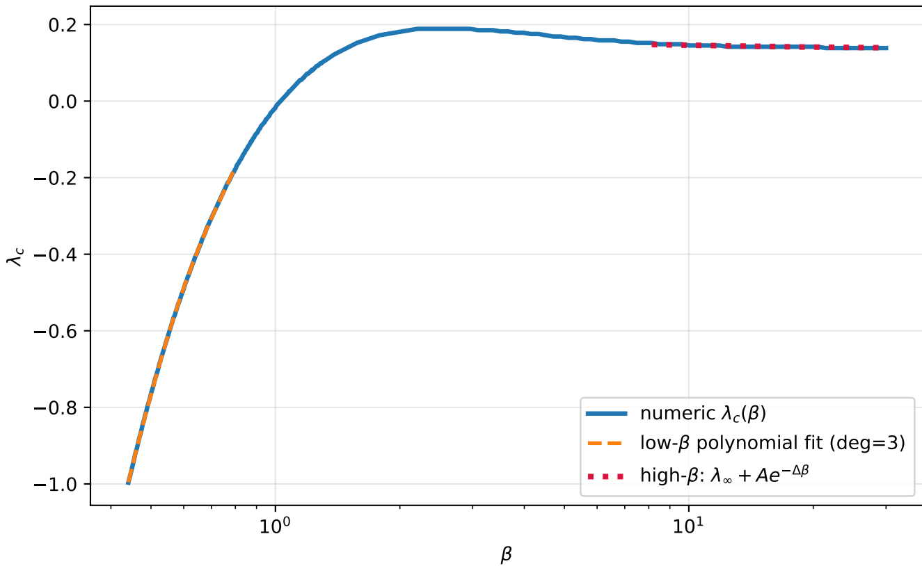
Concurrence: \lambda_c(\beta) with asymptotics
