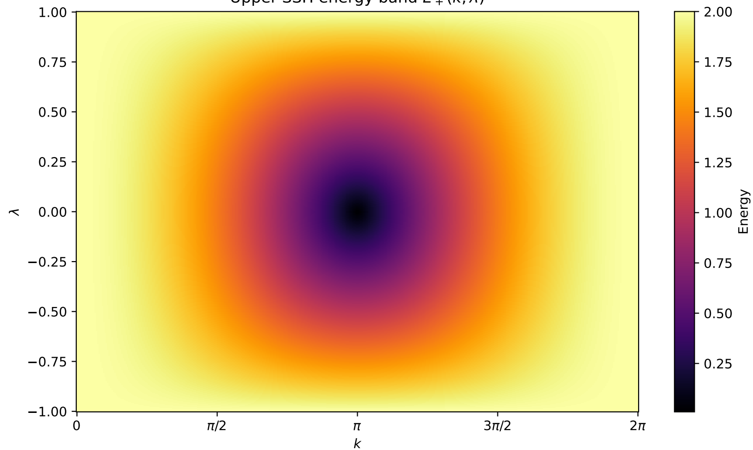
Upper SSH energy band E_+(k, \lambda)
