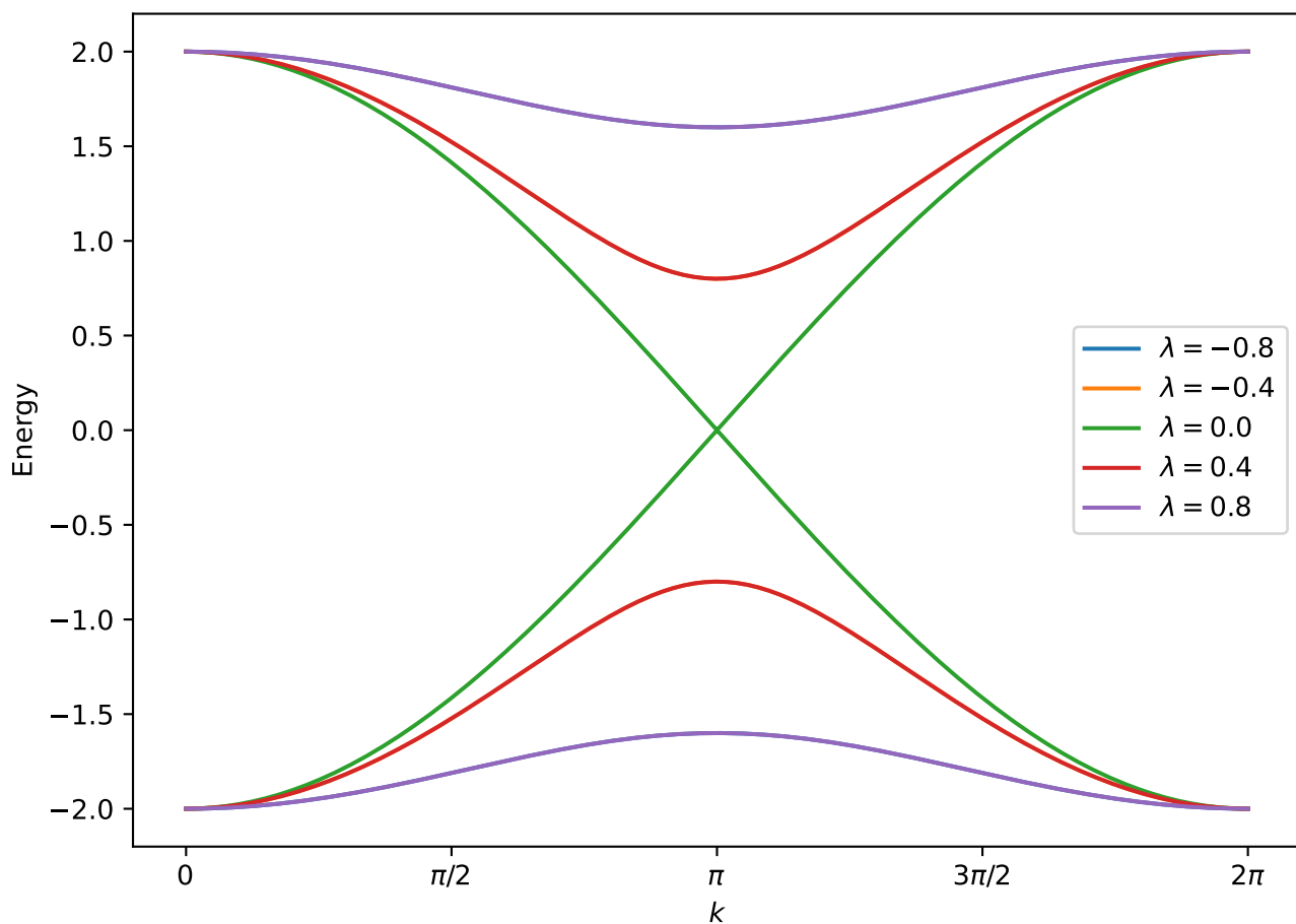
Upper SSH energy band E_+(k, \lambda)
