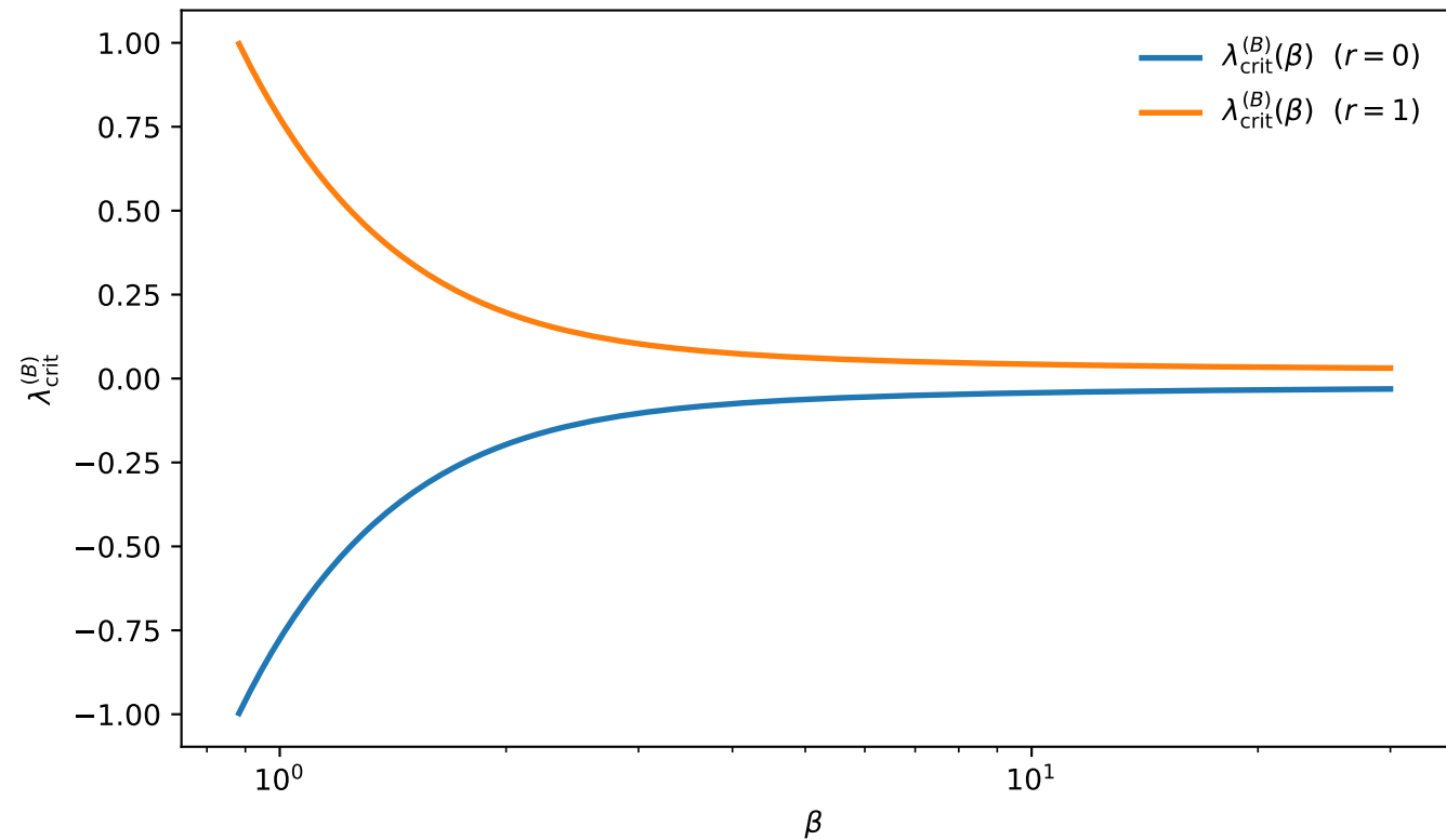
Critical line from Bell threshold \langle B \rangle = 2
