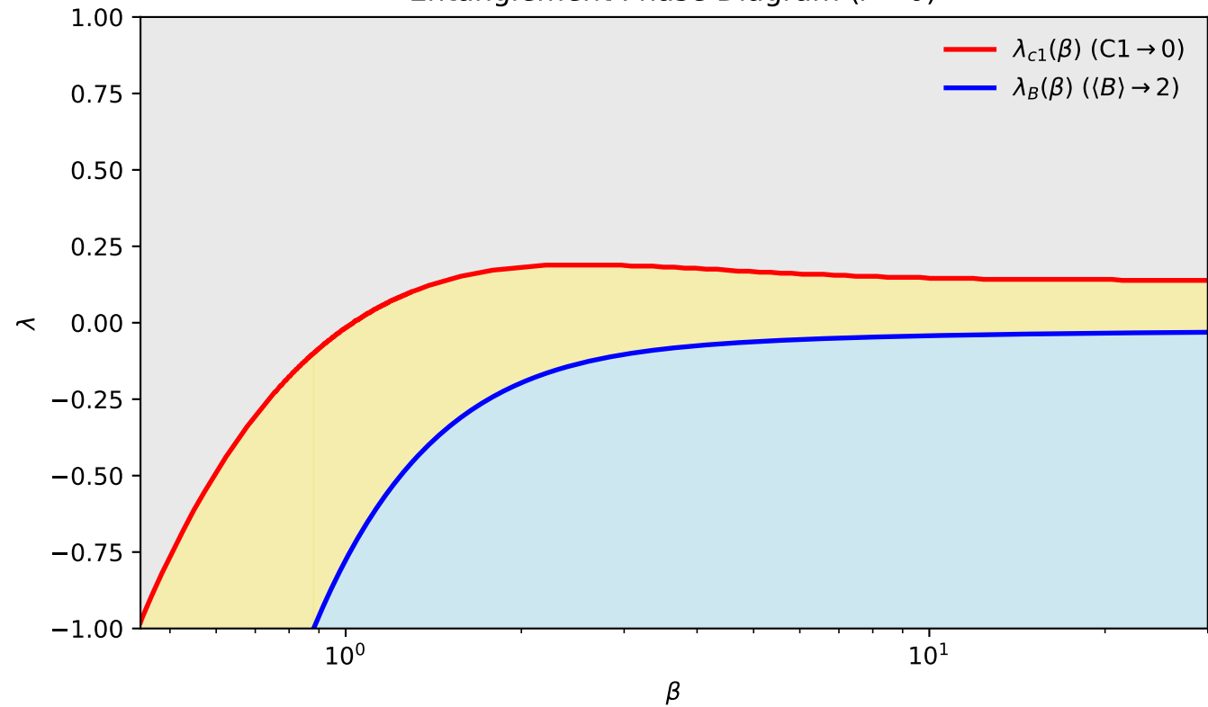
Entanglement Phase Diagram ( r = 0 )
