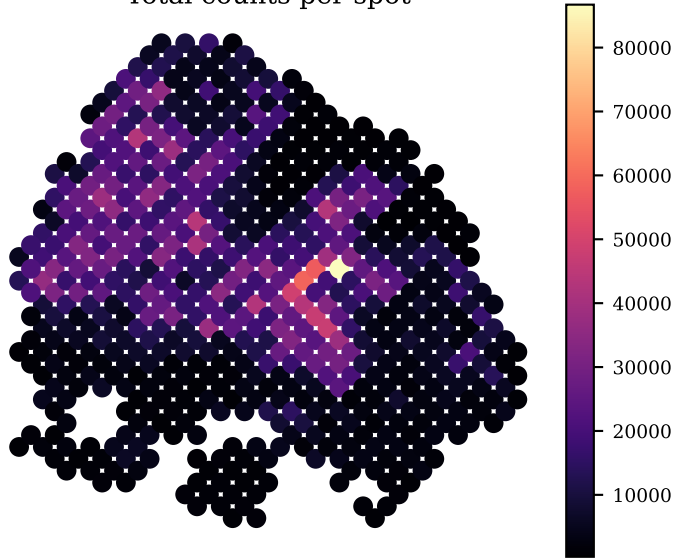
Total counts per spot
