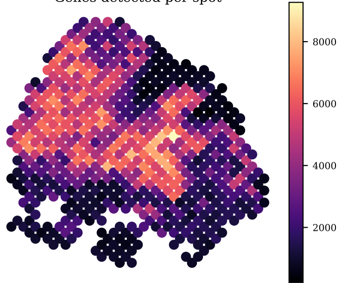
Genes detected per spot
