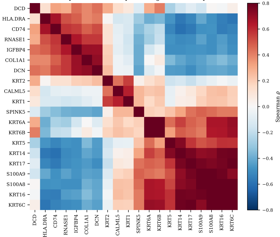
Co-expression of the top-ranked genes across spots
