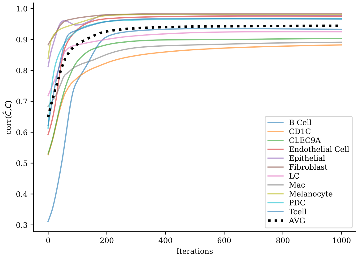
Gene-weight optimisation: correlation per cell type
