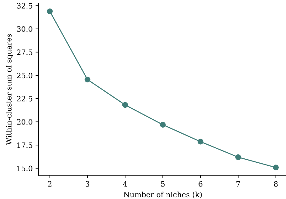
Elbow
