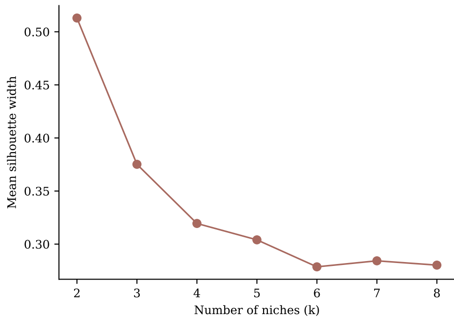
Silhouette
