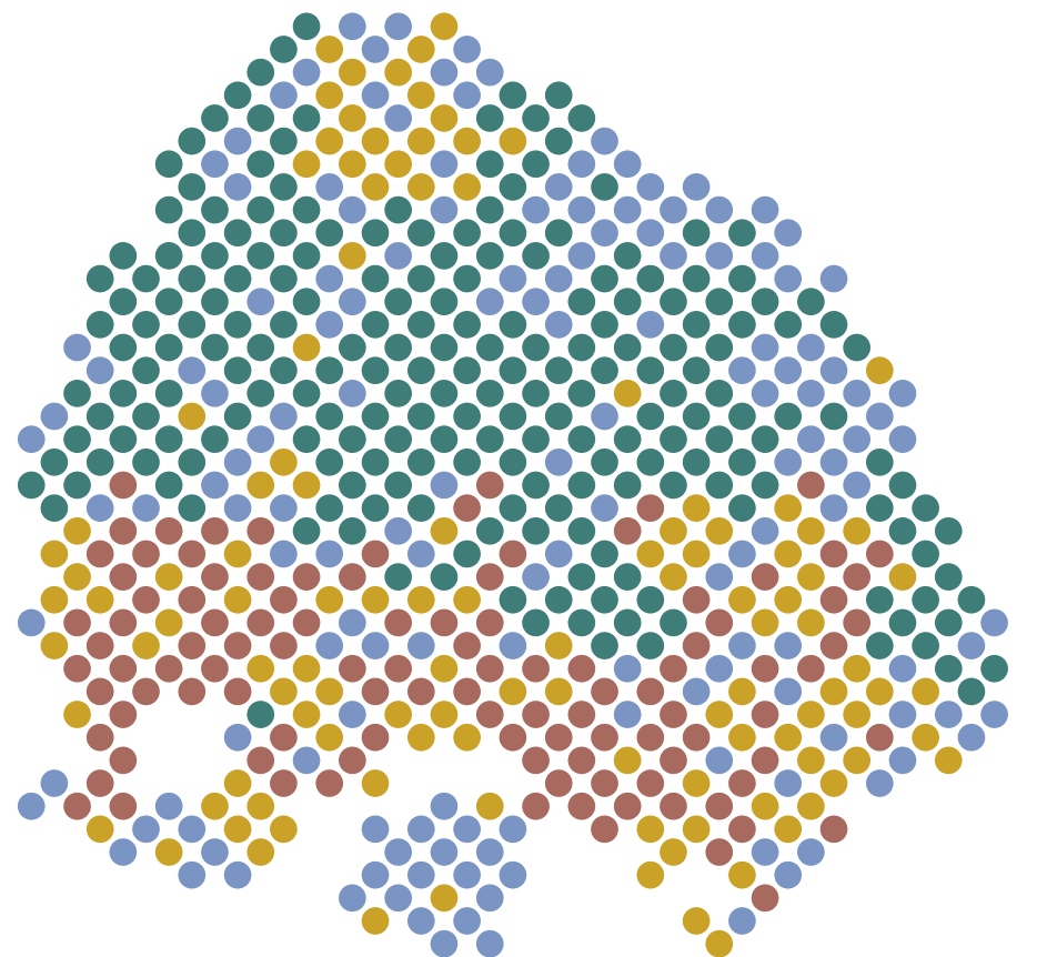
Spatial distribution of composition-defined niches
