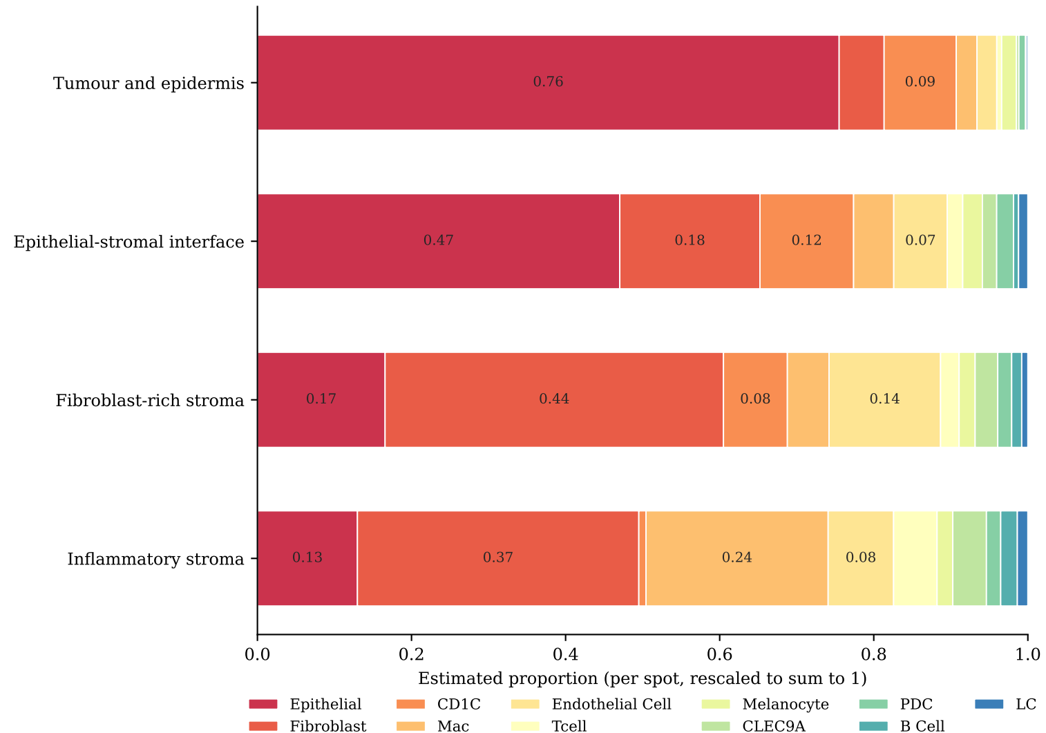
Mean cell-type composition per niche
