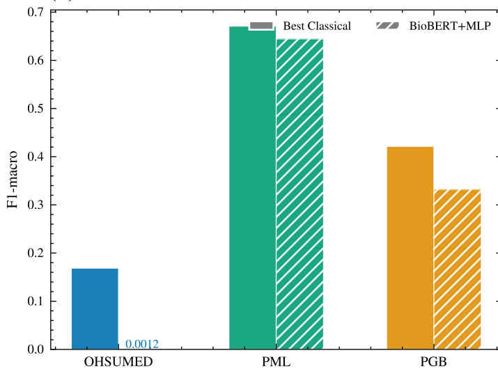
(A) BioBERT+MLP vs Best Classical
