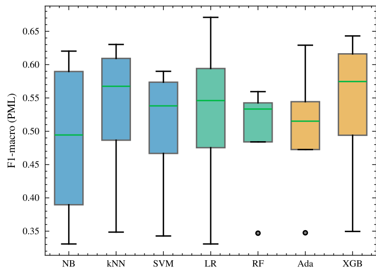
(D) Model Robustness Across Features
