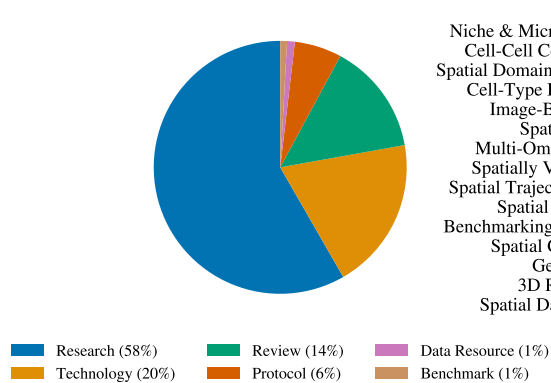
(B) Category
