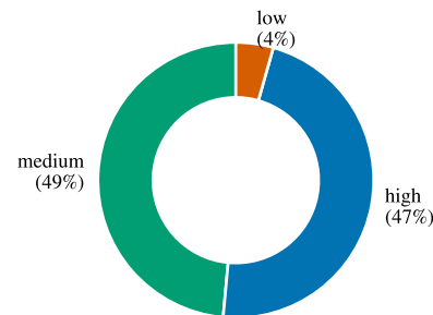
(H) Confidence
