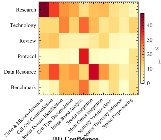
(H) Confidence
