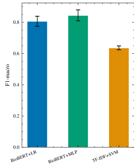
(A) ST Benchmark
