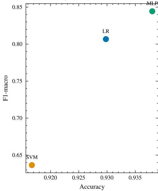
(C) Accuracy vs F1-macro
