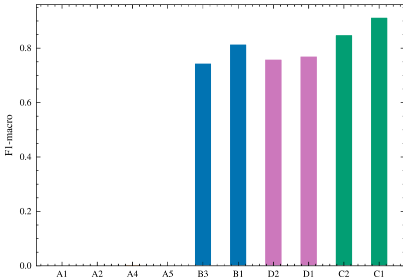
(A) Transfer Learning Waterfall
