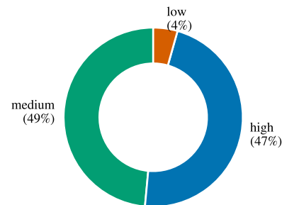
(H) Confidence
