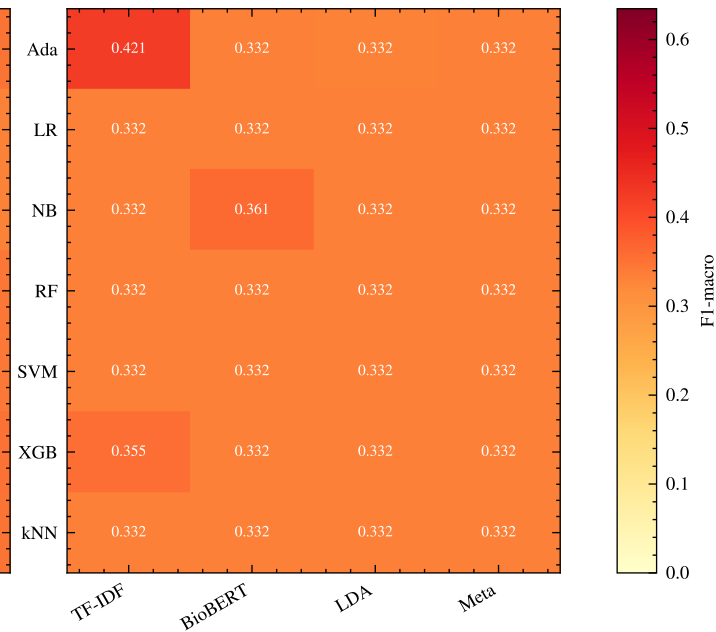
(C) PGB (3 labels)
