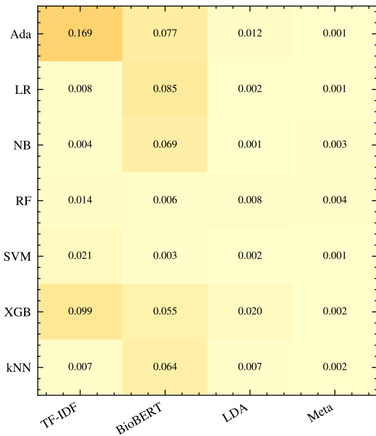
(A) OHSUMED (1,650 labels)
