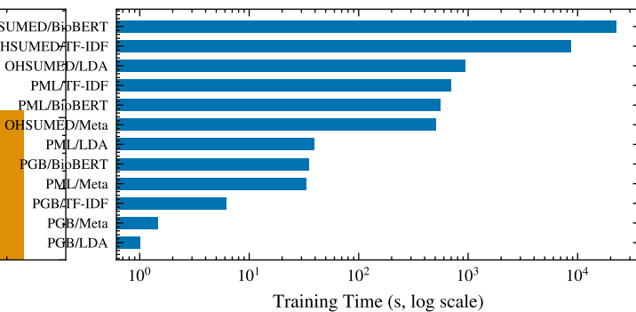
(E) Training Time by Feature × Dataset
