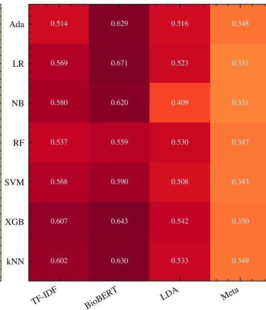
(B) PubMed-MultiLabel (16 labels)
