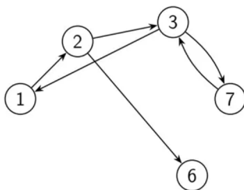
图 2: 4-2 Problem
