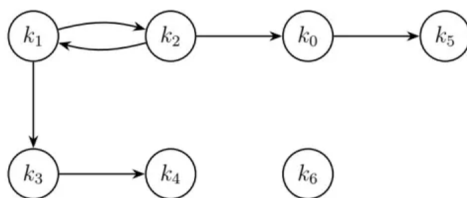
图 1: 4-1 Solution
